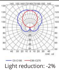
PHOTOMETRIC CURVE
