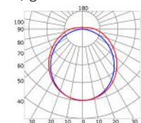
Transparent cover (light reduction: -4%)
